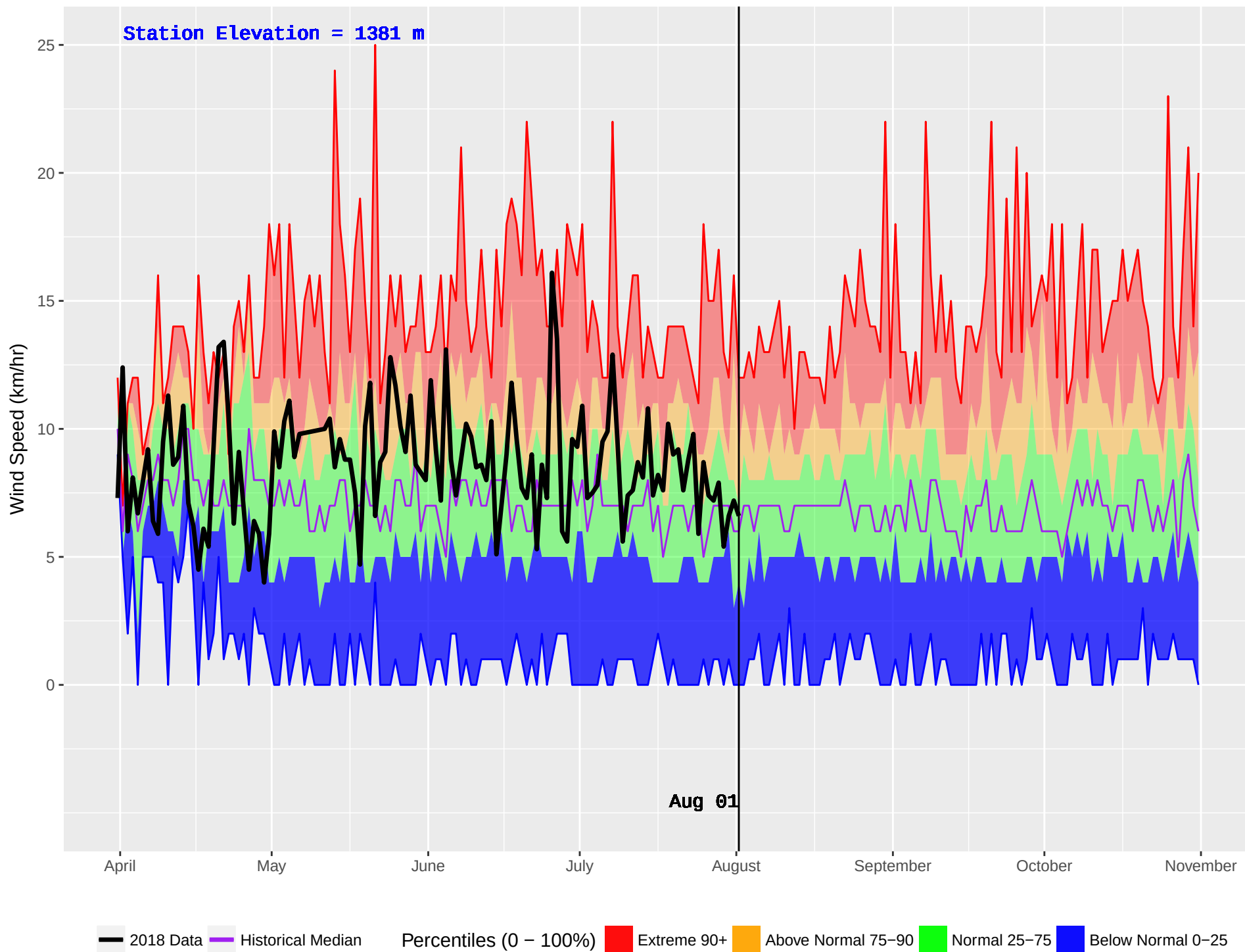
GLIMPSE (291) : Historical (1978–2016) and Current (2018) Daily Wind Speed
