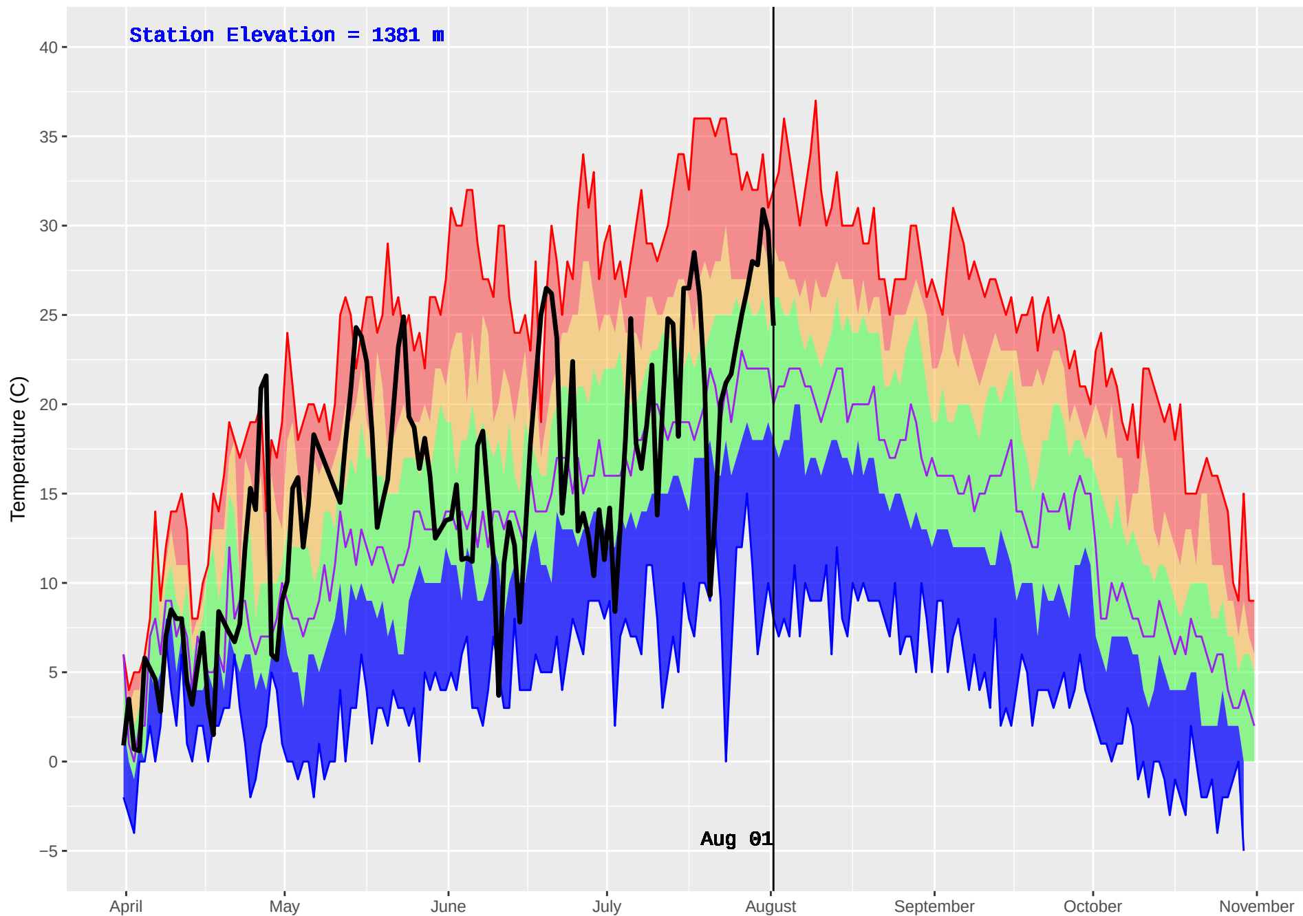
GLIMPSE (291) : Historical (1978–2016) and Current (2018) Daily Temperature
